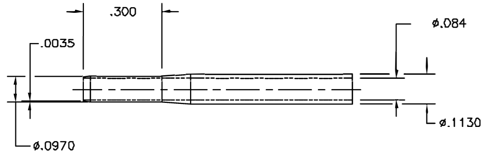
PROBE DETAIL
